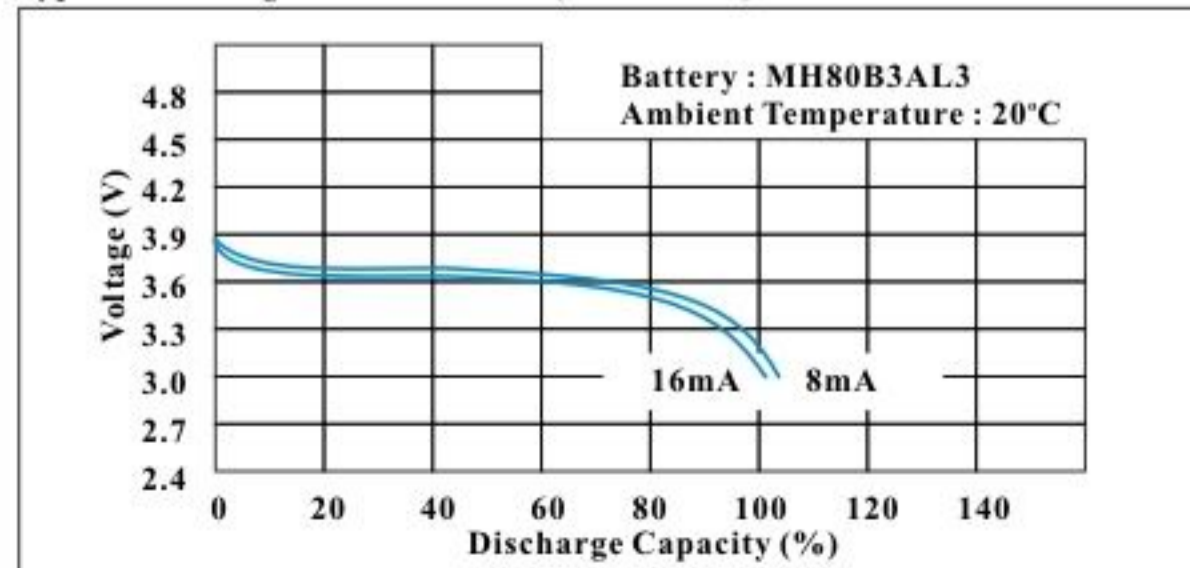
Typical Discharge Characteristics (Button Cell)
