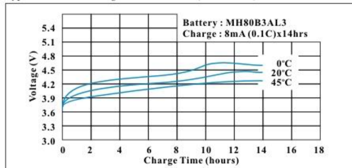
Typical Quick Charge Characteristics (Button Cell)
