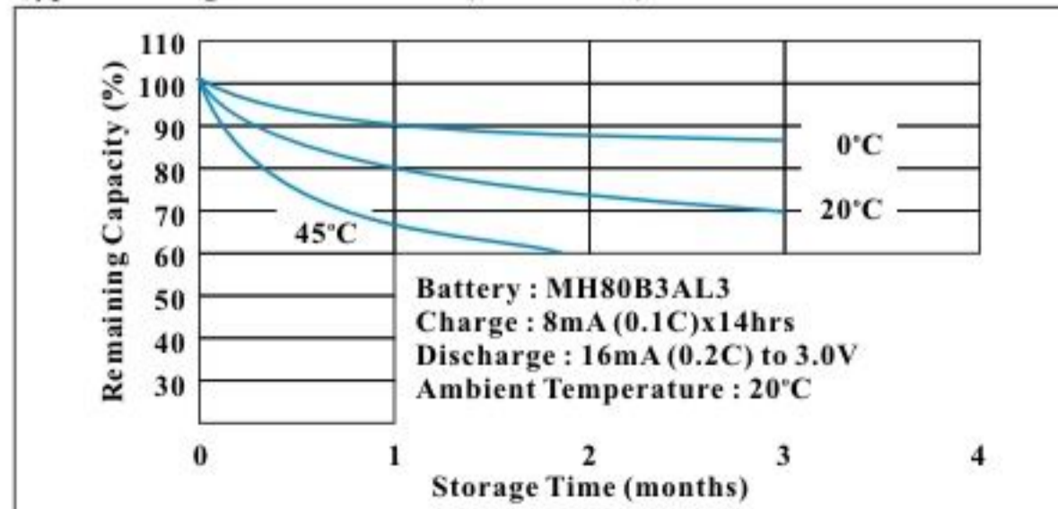
Typical Storage Characteristics (Button Cell)
